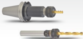
P.176 ER Spring Collet Chuck 177 彈性筒夾本體 BT/Straight Shank series
