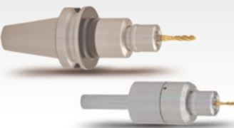
P.055 WASK Synchro Tap Holder 同步攻牙本體 BT/Straight Shank series
